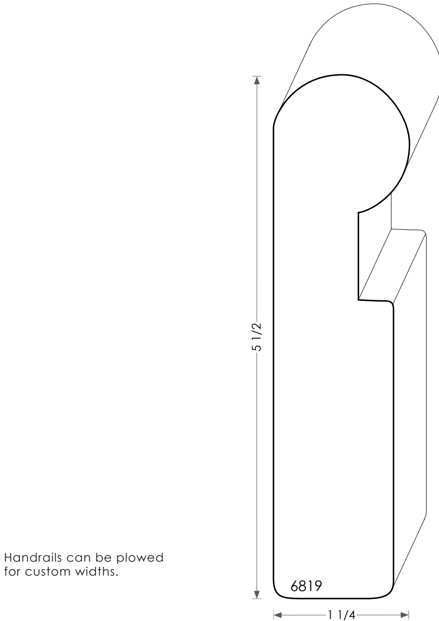
Wood Handrail - 6819
