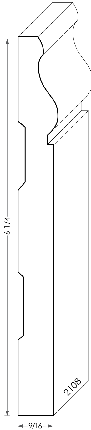
Wood Baseboard - 2108
