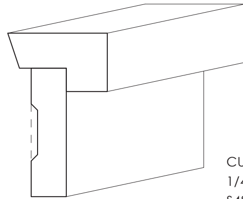
NOTCHED S4S [1-1/4 X 2-1/4] S4S [3/4 X 2-1/2]
