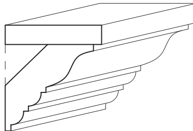
CUSTOM S4S [7/16 x 2]
