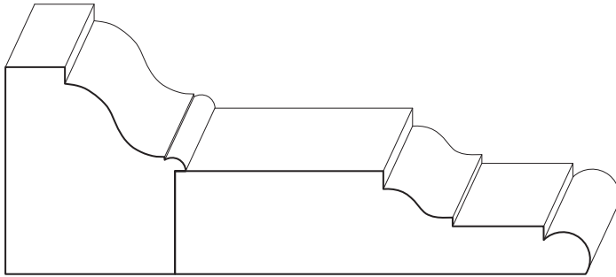
CUSTOM BACKBAND [2-1/2 X 2-1/8]
