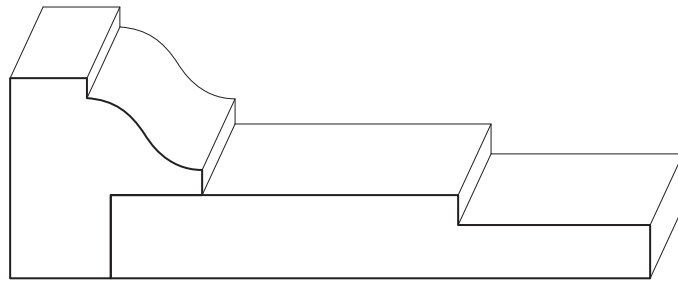
CUSTOM BACKBAND [2 X 2] CUSTOM CASING [7/8 X 5-1/2]
