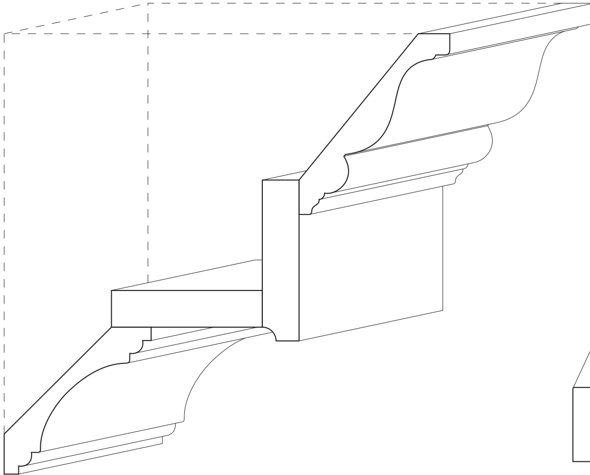
3078 [ \frac{3}{4} X 4- \frac{3}{4} ] S4S COVE [ \frac{3}{4} X 3- \frac{1}{4} ] S4S [ \frac{3}{4} X 3] 3034 [ \frac{3}{4} X 4- \frac{3}{16} ]
