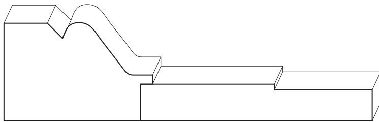
CUSTOM CASING [3/4 X 4-7/8] CUSTOM BACKBAND [2 X 3]
