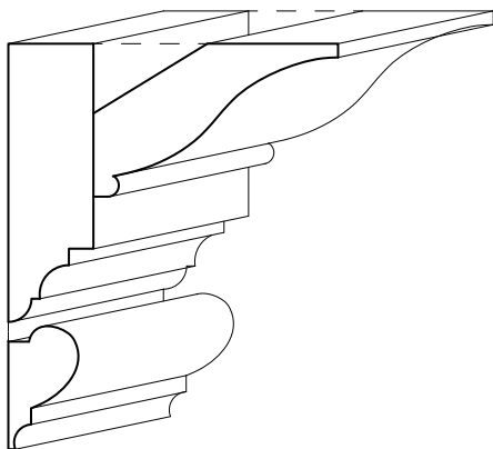
CUSTOM MOLD [3/4 X 2-5/8]
