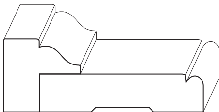
7034 MODIFIED [1-9/16 x 1-5/8] 1144 [13/16 x 2-7/8]
