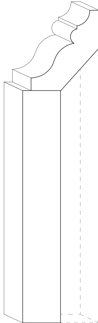
CUSTOM CROWN [1-1/8 X 4-3/32]
