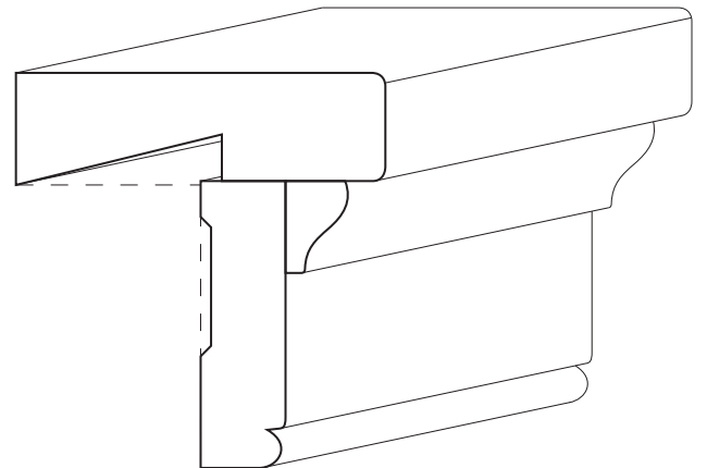
9002 [1-1/16 X 3-1/2] 5732 [9/16 X 13/16] 1144 [13/16 X 2-3/4]
