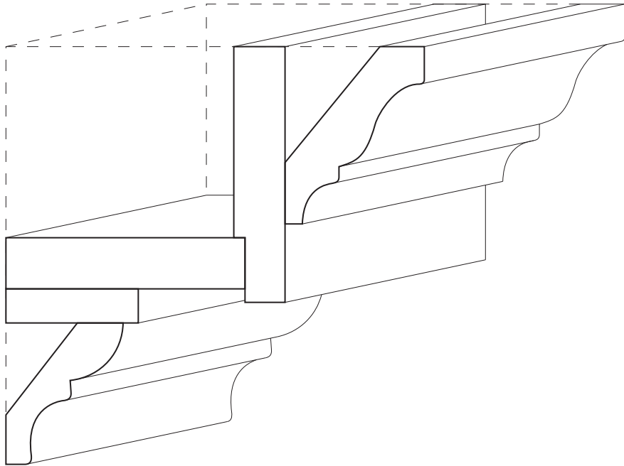
3082 [11/16 X 2-5/8] S4S W/ NOTCH [3/4 X 3-3/4] S4S [3/4 X 3-1/2] S4S [1/2 X 2] 3052 [3/4 X 3-1/4]
