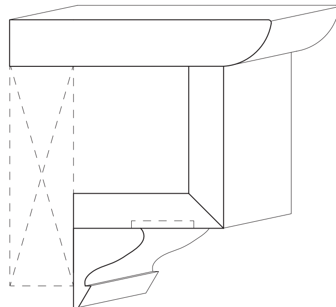
CUSTOM MOLD [1 X 5-3/4]
